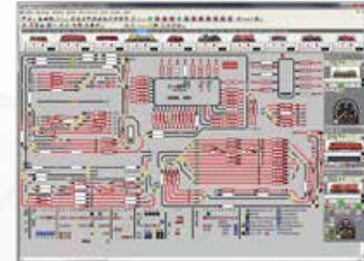
WinDigipet
